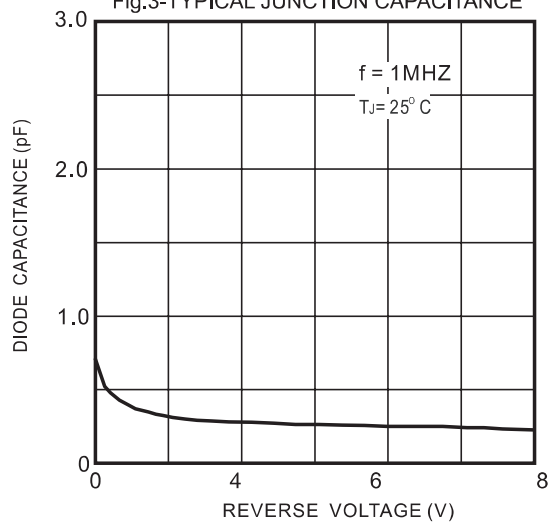
Fig.3-TYPICAL JUNCTION CAPACITANCE
