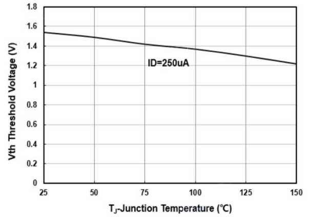
Figure8. Threshold Voltage vs Temperature
