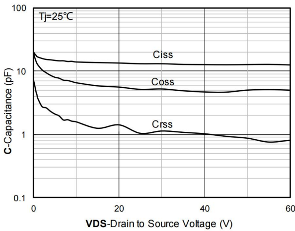
Figure 3. Capacitance Characteristics
