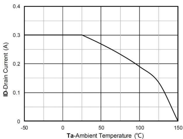
Current dissipation
