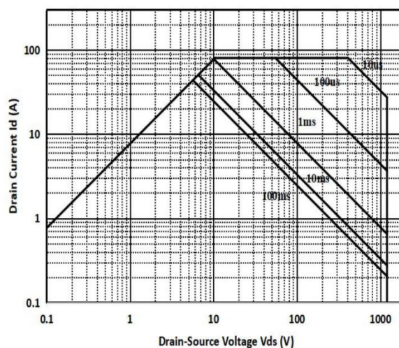
Figure 18. Safe Operating Area
