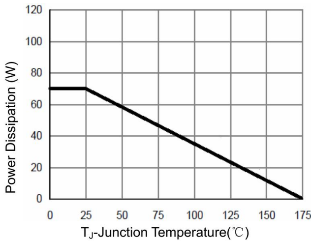
Figure 9 Power De-rating
