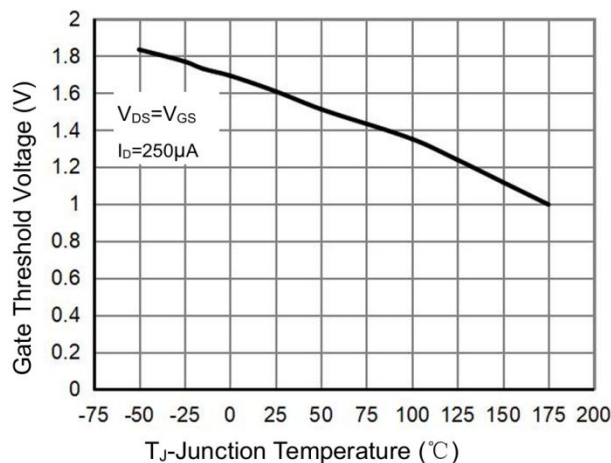
Figure 12 V_{GS(th)} -Junction Temperature
