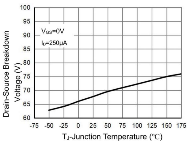
Figure 11 BV_{DSS} -Junction Temperature
