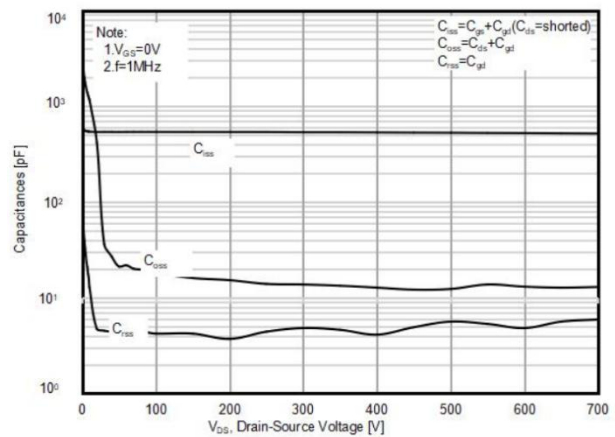
Figure10. Capacitance
