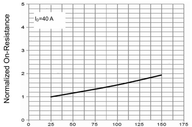
T J -Junction Temperature(°C) Figure 10 Rdson-Junction Temperature
