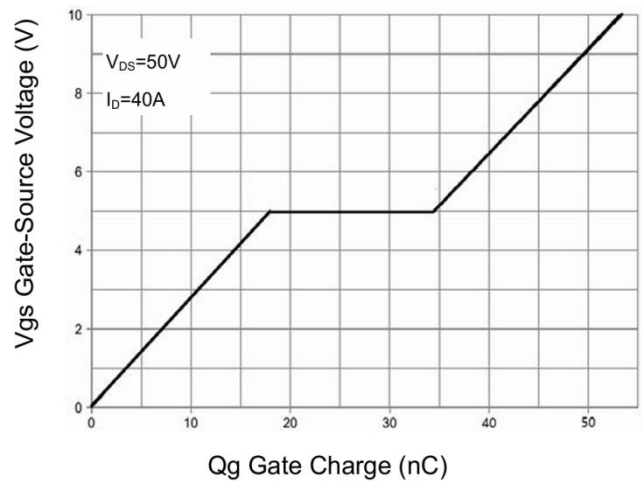
Figure 4 Gate Charge
