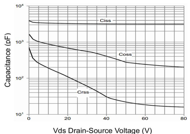
Figure 6 Capacitance vs Vds
