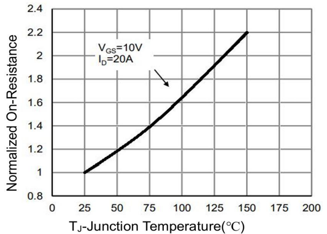
Figure 4 Rdson-Junction Temperature
