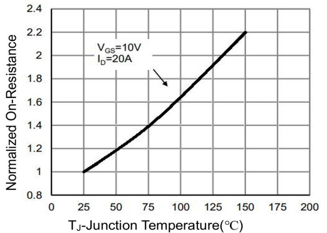
Figure 4 Rdson-Junction Temperature
