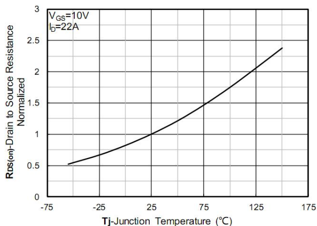
Figure 6. Normalized On-Resistance
