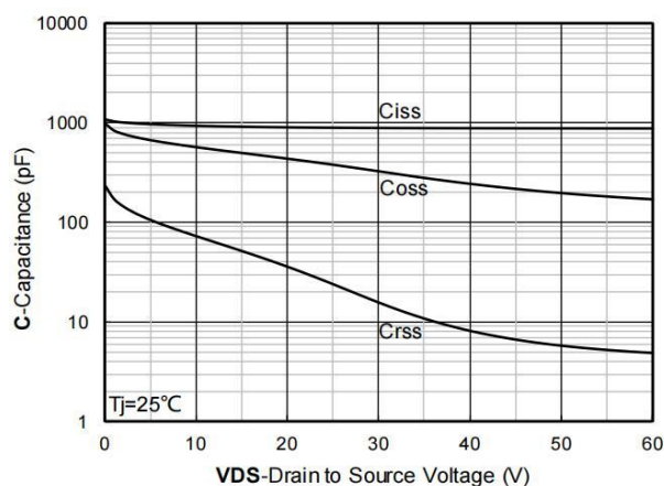
Figure 3. Capacitance Characteristics
