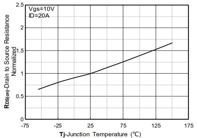
Figure 6. Normalized On-Resistance
