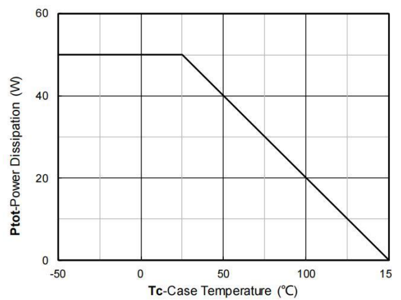
Figure 12. Power dissipation
