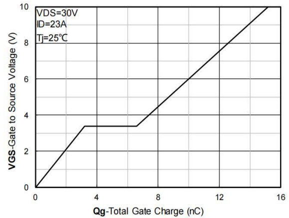
Figure 4. Gate Charge
