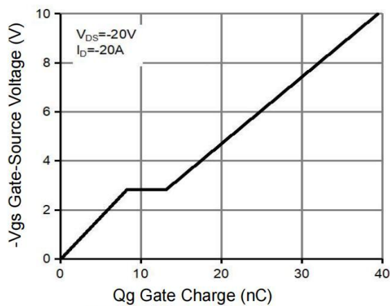
Figure 5 Gate Charge
