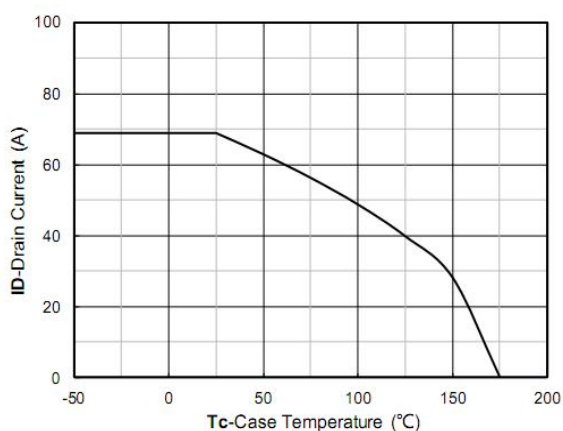
Figure 11. Current dissipation
