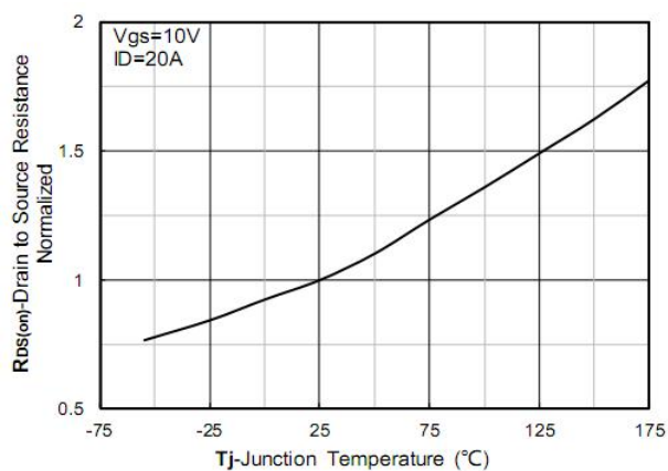
Figure 6. Normalized On-Resistance
