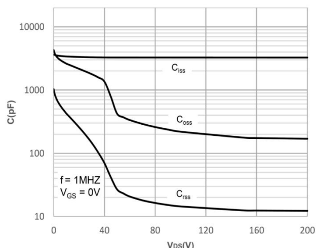
Capacitance Characteristics
