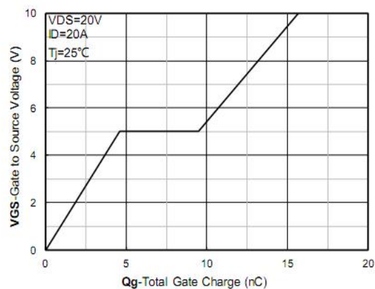
Figure 4. Gate Charge
