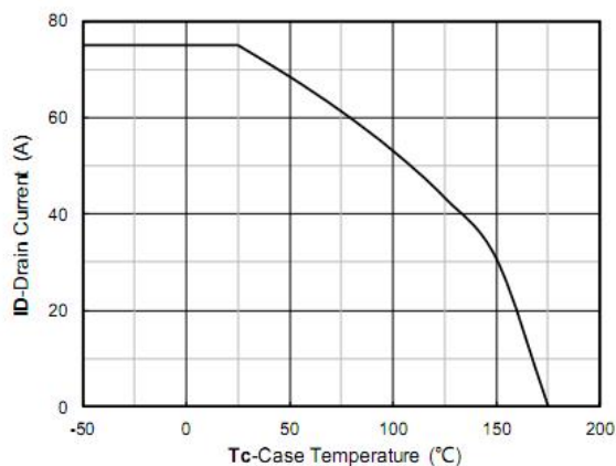
Figure 11. Current dissipation
