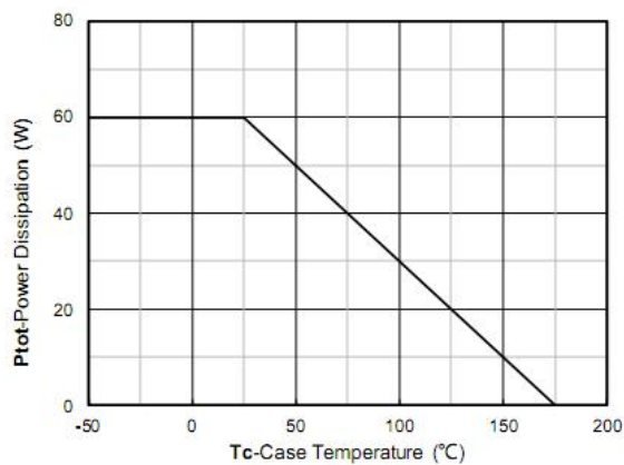
Figure 12. Power dissipation
