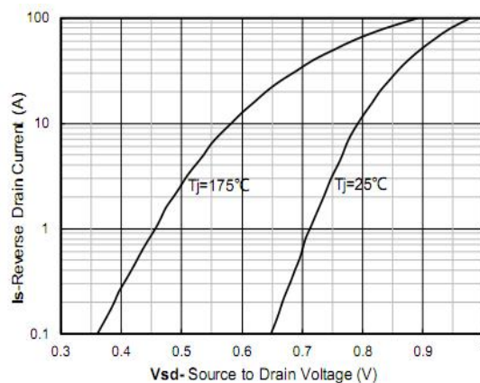
Figure 8. Forward characteristics of reverse diode
