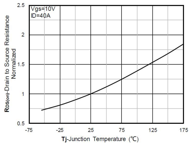
Figure 6. Normalized On-Resistance
