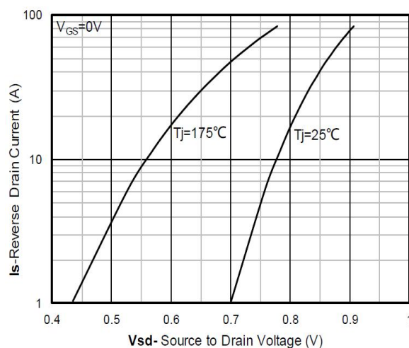
Figure 8. Forward characteristics of reverse diode
