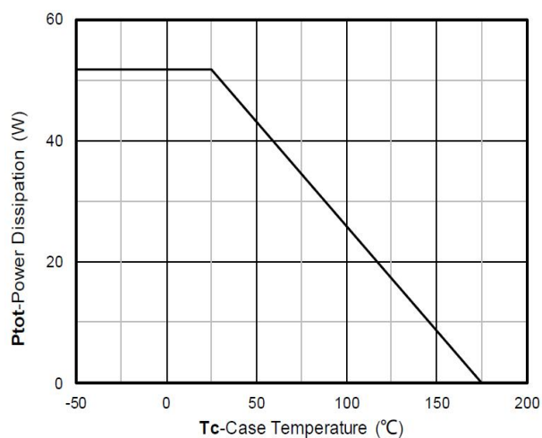
Figure 12. Power dissipation
