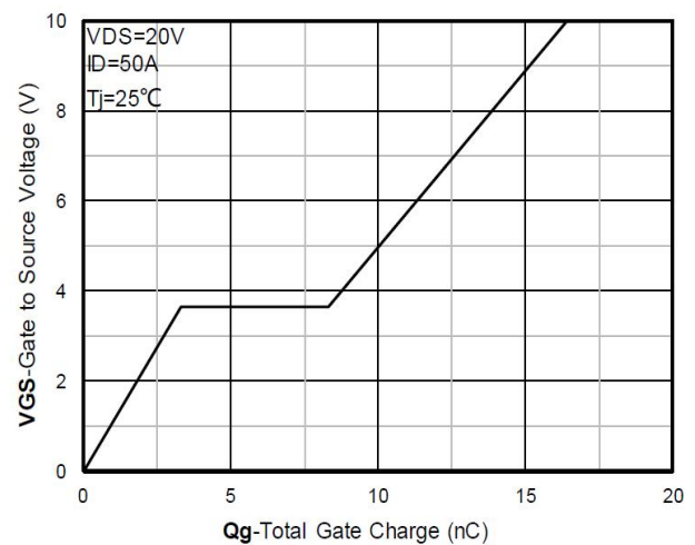
Figure 4. Gate Charge
