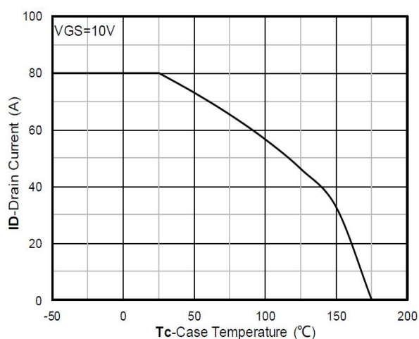
Figure 11. Current dissipation
