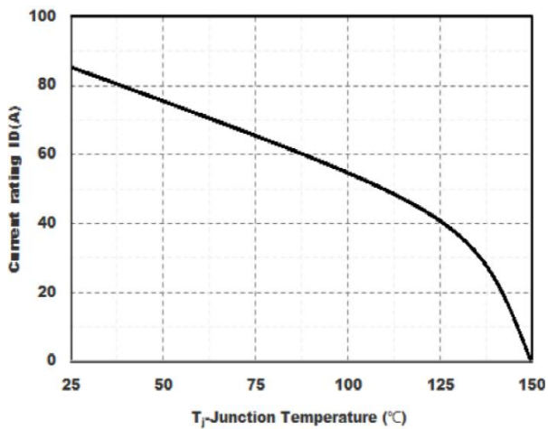
Figure7. Drain current
