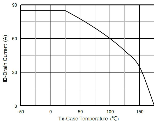
Figure 11. Current dissipation
