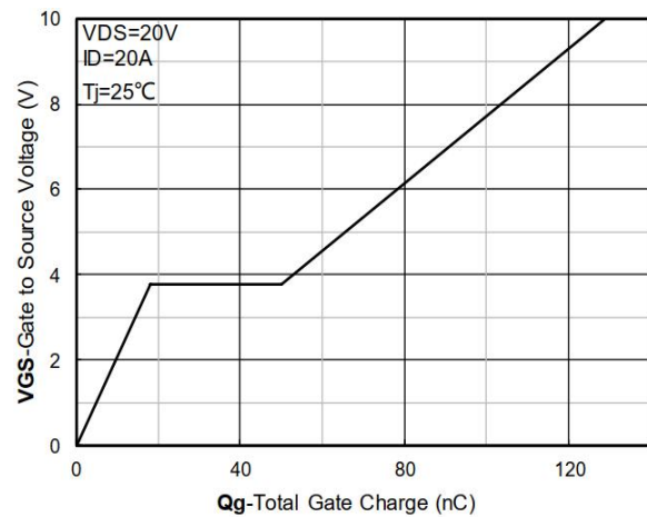
Figure 4. Gate Charge
