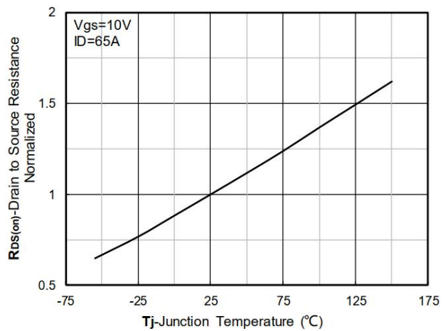
Figure 6. Normalized On-Resistance
