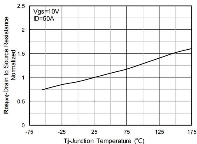
Figure 6. Normalized On-Resistance
