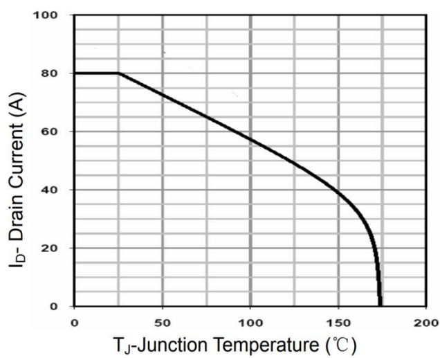
Figure 10 Current De-rating
