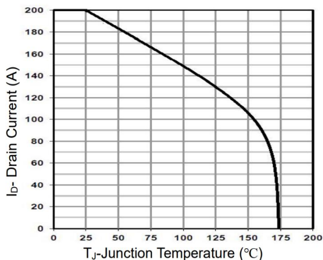
Figure 10 Current De-rating
