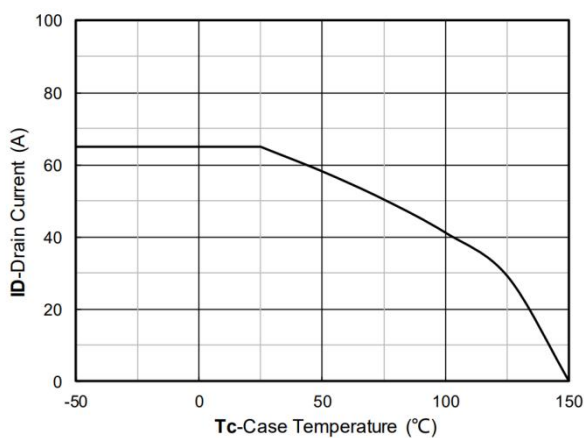
Figure 11. Current dissipation
