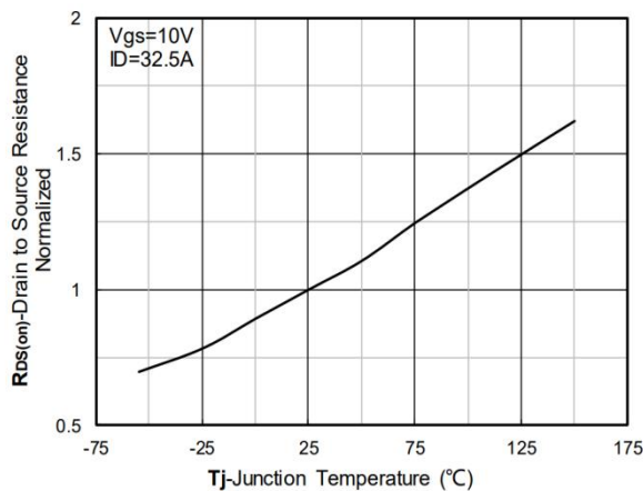
Figure 6. Normalized On-Resistance
