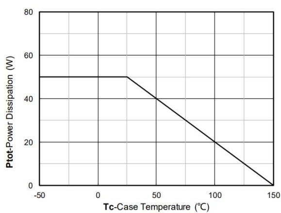
Figure 12. Power dissipation
