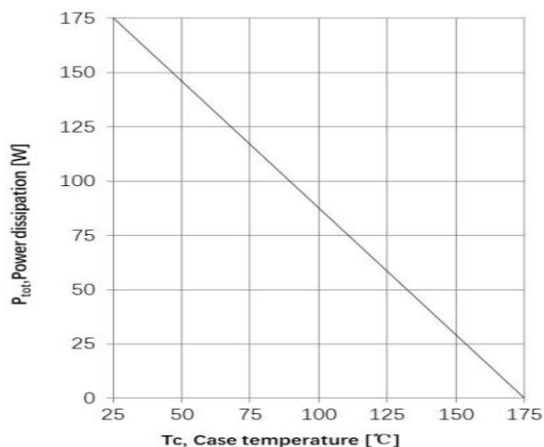
Fig1. Power dissipation as a function of case temperature ( T_i \leq 175^\circ\text{C} )
