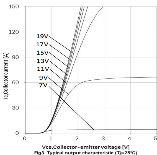
Fig3. Typical output characteristic ( T_j = 25^\circ\text{C} )
