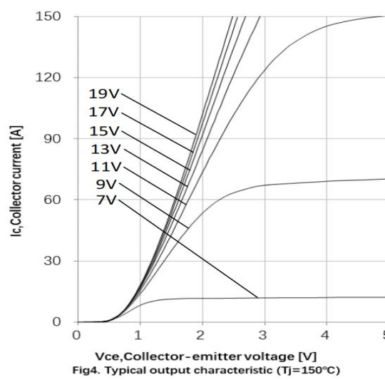
Fig4. Typical output characteristic ( T_j = 150^\circ\text{C} )
