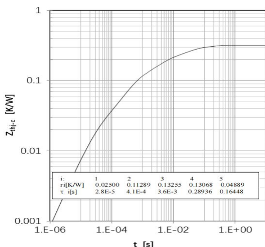
Fig 15. IGBT Transient Thermal Impedance
