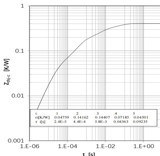
Fig 16. Diode Transient Thermal Impedance
