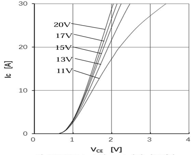
Fig2.IGBT Output Characteristics(150°C)
