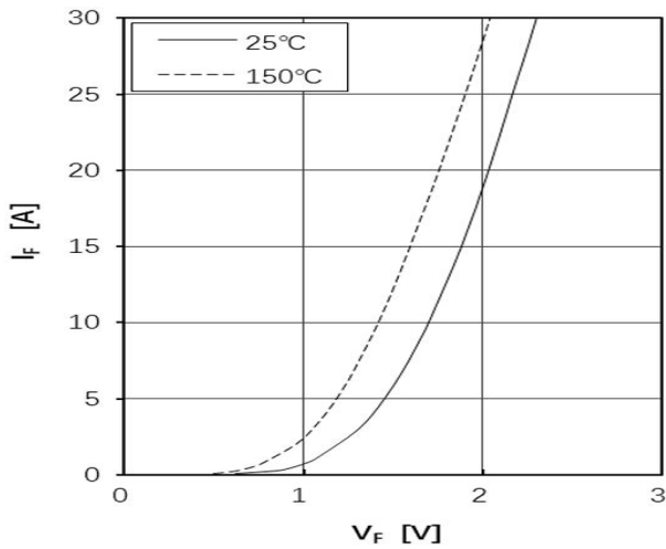
Fig3.Diode Foward Characteristics
