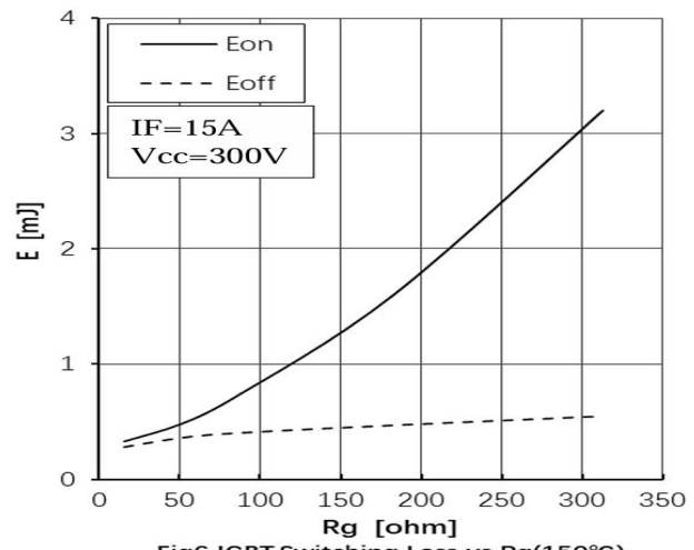
Fig6.IGBT Switching Loss vs.Rg(150°C)
