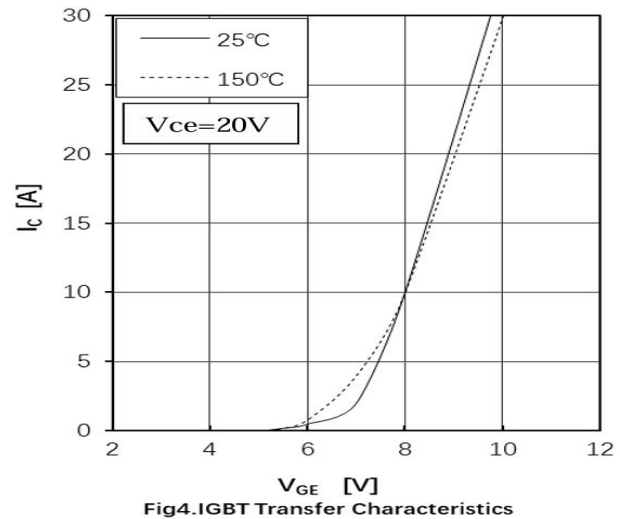
Fig4.IGBT Transfer Characteristics
