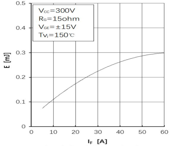
Fig8. Diode Switching Loss( E_{rec} ) vs. I_F
