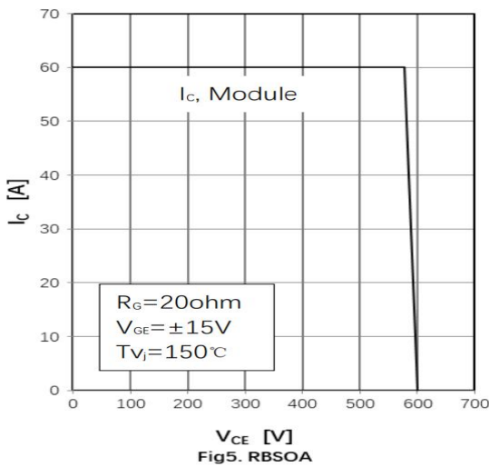
Fig5. RBSOA
