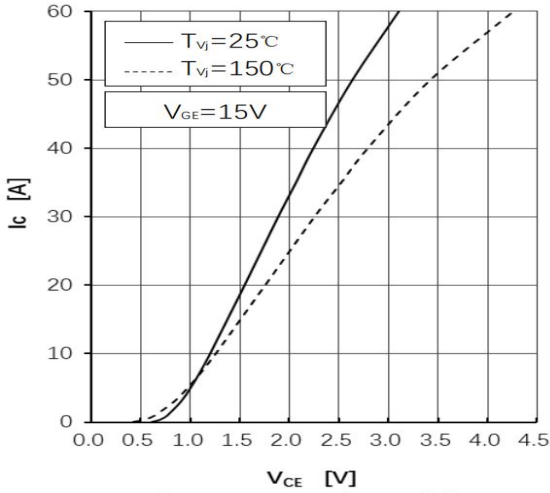
Fig1.IGBT Output Characteristics
