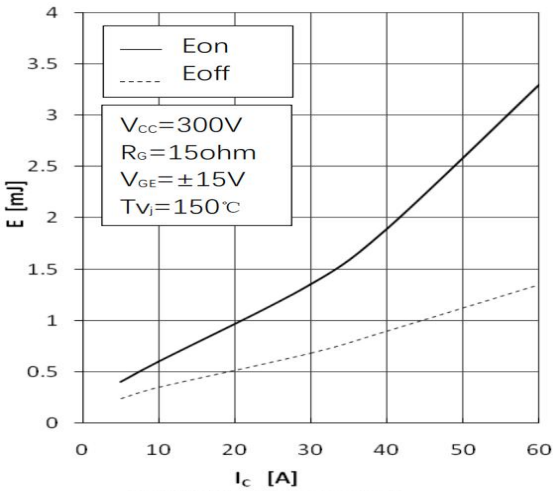
Fig3.IGBT Switching Loss vs.Ic
