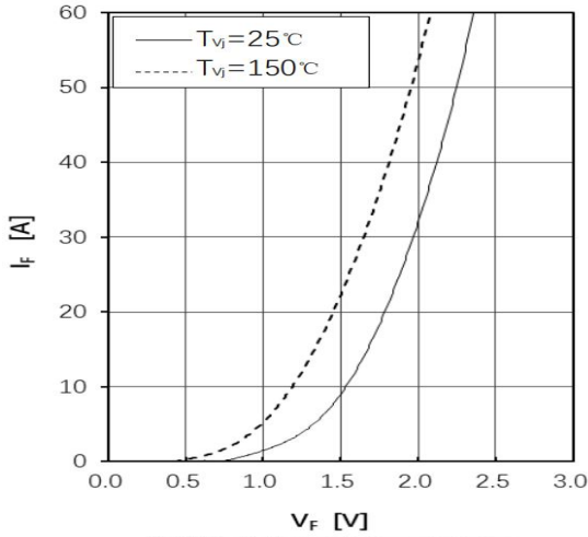
Fig7. Diode Forward Characteristics
