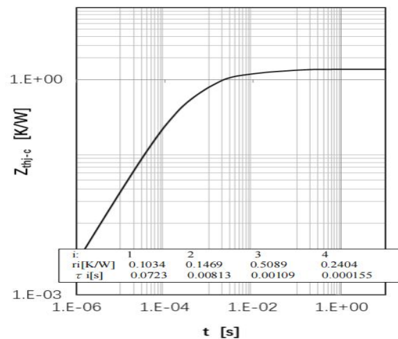
Fig 10. Diode Transient Thermal Impedance
