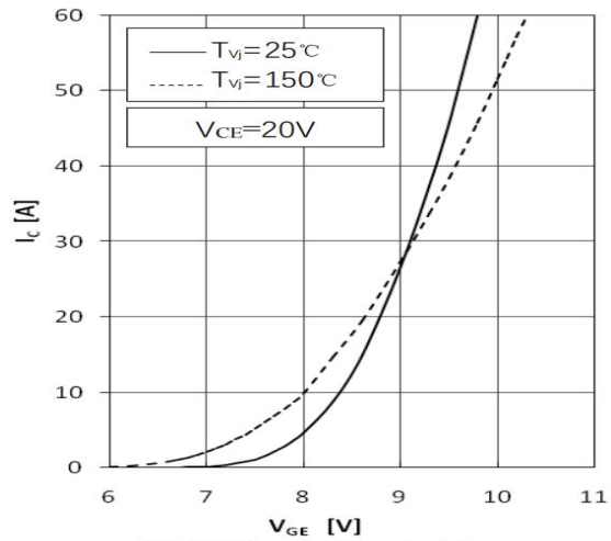
Fig2.IGBT Transfer Characteristics
