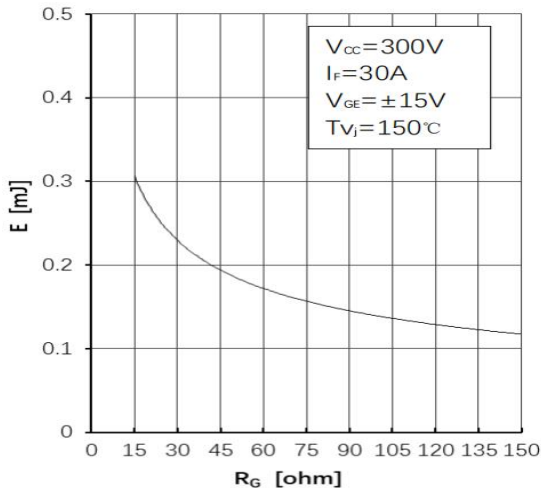
Fig9. Diode Switching Loss( E_{rec} ) vs. R_G
