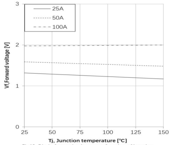
Fig18. Diode forward voltage as a function of junction temperature
