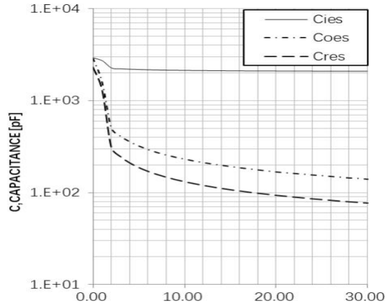
Fig16. Typical capacitance as a function of collector-emitter voltage
