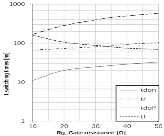
Fig8. Typical switching times as a function of gate resistance (inductive) load, T_{vj}=150^{\circ}\text{C} , V_{ce}=400\text{V} , V_{ge}=0/15\text{V} , I_c=60\text{A}
