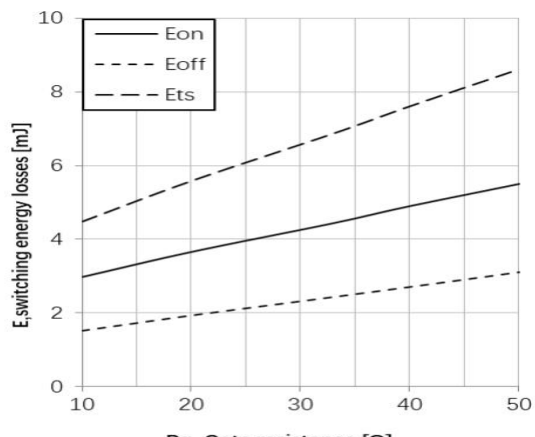
Fig12. Typical switching energy losses as a function of gate resistance (inductive) load, T_{vj}=150^{\circ}\text{C} , V_{ce}=400\text{V} , V_{ge}=0/15\text{V} , I_c=60\text{A}
