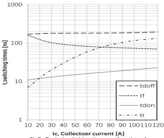
Fig7. Typical switching time as a function of collector current (inductive) load, T_{vj}=150^{\circ}\text{C} , V_{ce}=400\text{V} , V_{ge}=0/15\text{V} , R_g=10\Omega
