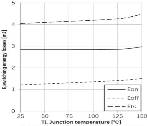
Fig13. Typical switching energy losses as a function of junction temperature (inductive) load, Ic=60A, Vce=400V, Vge=0/15V, Rg=10Ω
