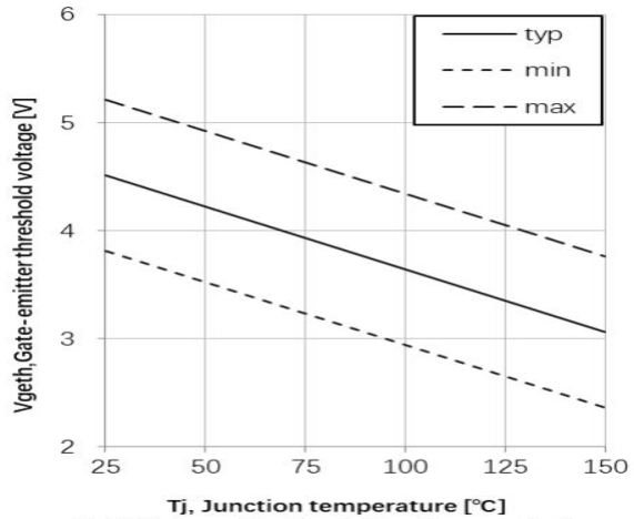
Fig10. Gate-emitter threshold voltage as a function of junction temperature ( I_c=0.8\text{mA} )
