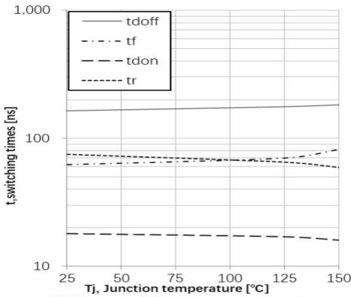
Fig9. Typical switching times as a function of junction temperature (inductive) load, I_c=60\text{A} , V_{ce}=400\text{V} , V_{ge}=0/15\text{V} , R_g=10\Omega
