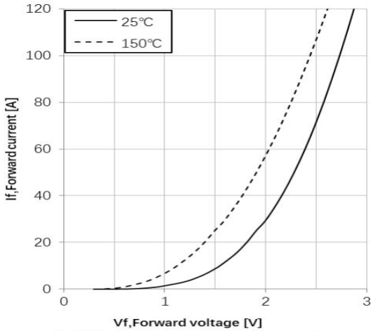
Fig19. Diode forward current as a function of forward voltage
