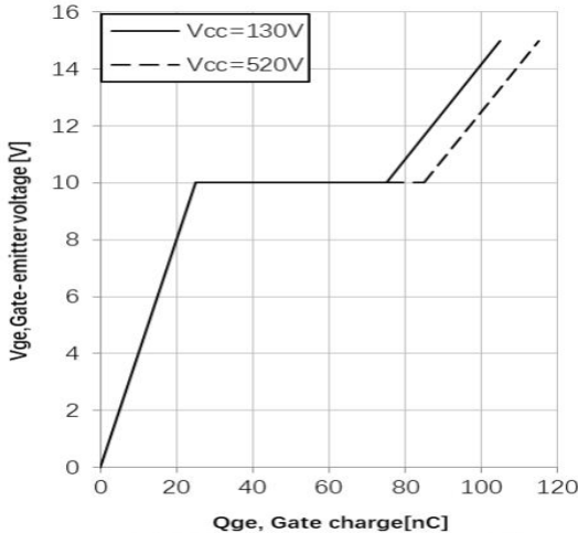
Fig15. Typical gate charge (Ic=60A)
