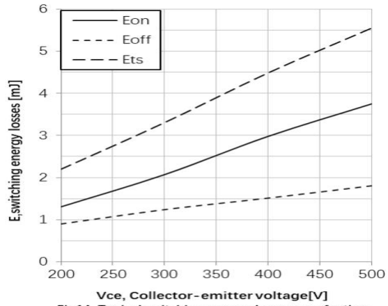
Fig14. Typical switching energy losses as a function of collector-emitter voltage (inductive) load, Tvj=150°C, Ic=60A, Vge=0/15V, Rg=10Ω
