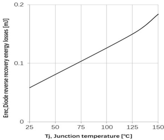
Fig21. Typical diode reverse recovery energy losses as a function of junction temperature (inductive load, I_f=60A, V_{rr}=400V )
