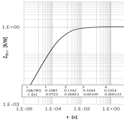
Fig 18. Diode Transient Thermal Impedance
