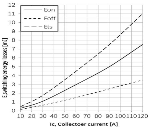
Fig11. Typical switching energy losses as a function of collector current (inductive) load, T_{vj}=150^{\circ}\text{C} , V_{ce}=400\text{V} , V_{ge}=0/15\text{V} , R_g=10\Omega
