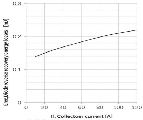
Fig22. Typical diode reverse recovery energy losses as a function of collector current (inductive load, T_{vj}=150^{\circ}C, V_{rr}=400V )
