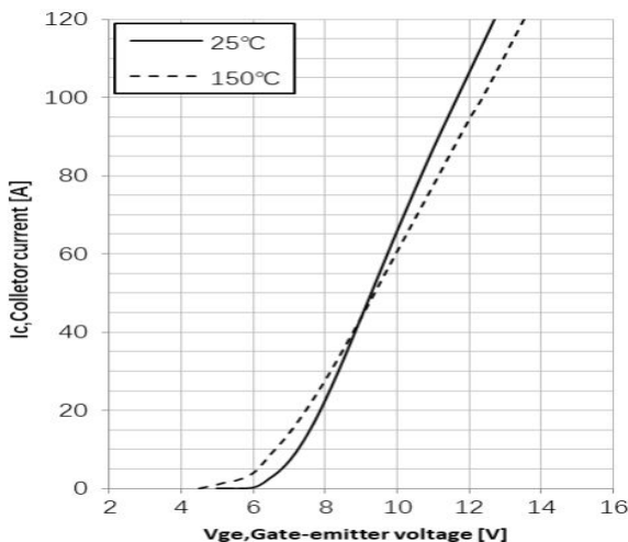
Fig5. Typical transfer characteristic ( V_{ce} = 20\text{V} )
