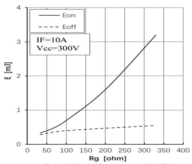
Fig6.IGBT Switching Loss vs. R_g (150°C)
