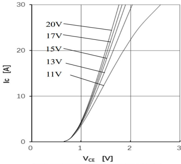
Fig1.IGBT Output Characteristics(25°C)
