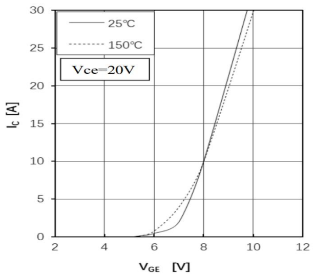
Fig4.IGBT Transfer Characteristics
