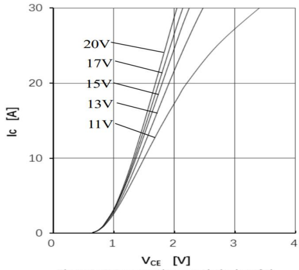
Fig2.IGBT Output Characteristics(150°C)
