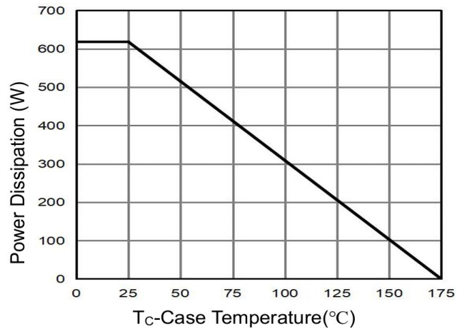
Figure 10 Power De-rating
