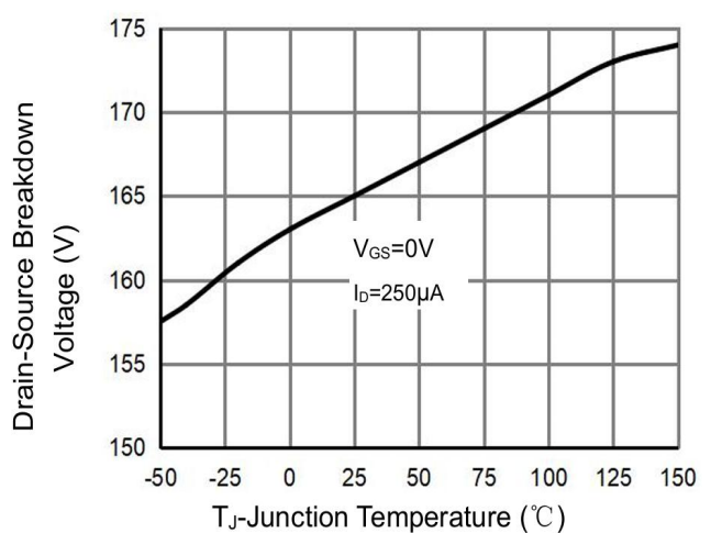
Figure 12 BV_{DSS} -Junction Temperature
