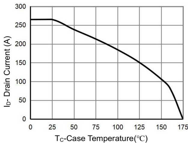
Figure 11 Current De-rating
