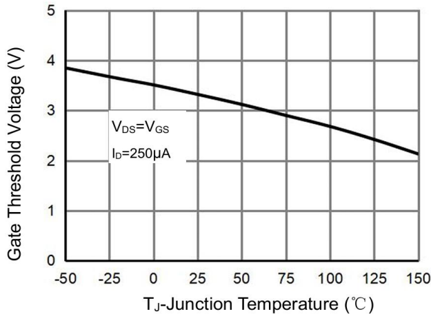
Figure 9 V_{GS(th)} -Junction Temperature
