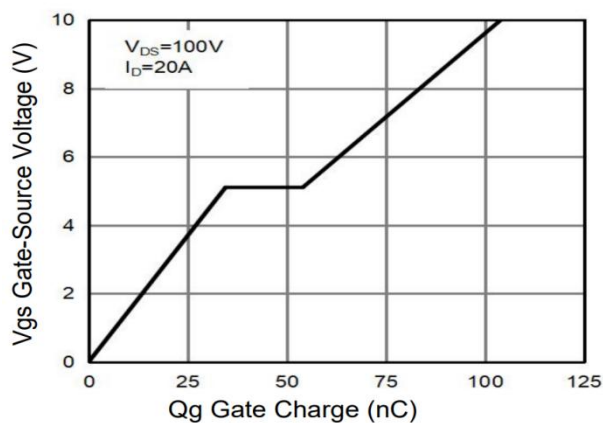
Figure 5 Gate Charge
