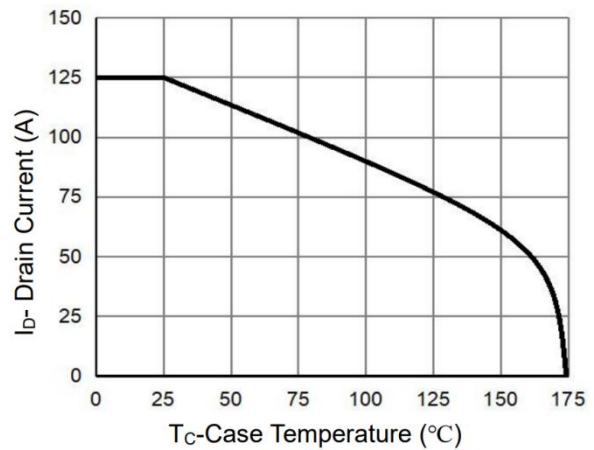
Figure 10 Current De-ratin
