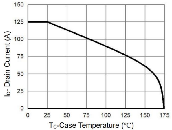
Figure 10 Current De-ratin
