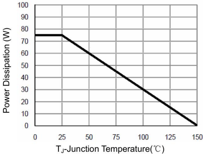
Figure 9 Power De-rating
