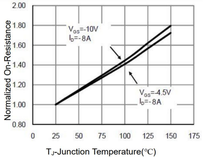
Figure 4 Rdson-Junction Temperature
