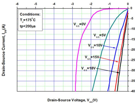
Figure 11. 3rd Quadrant Characteristic at 175°C
