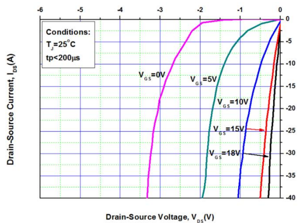
Figure 10. 3rd Quadrant Characteristic at 25°C
