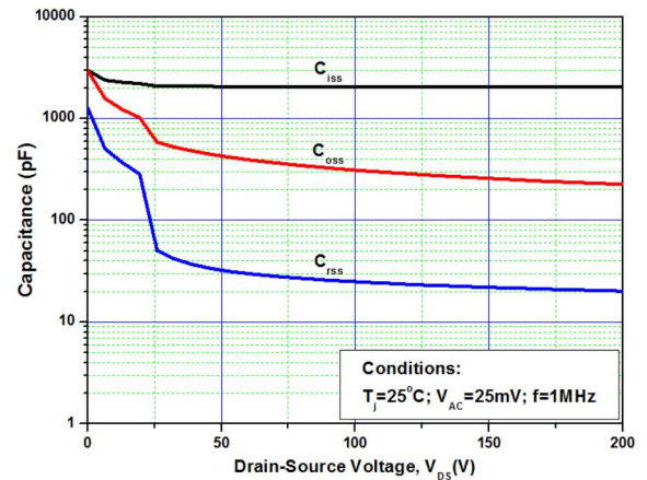
Figure 12. Capacitances vs. Drain-Source Voltage (0 - 200V)
