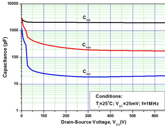
Figure 13. Capacitances vs. Drain-Source Voltage (0 - 650V)
