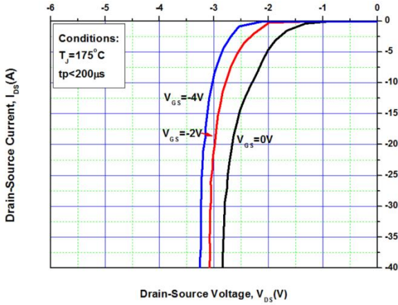
Figure 7. Body Diode Characteristic at 175°C
