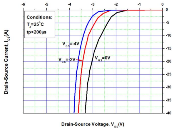
Figure 6. Body Diode Characteristic at 25^\circ\text{C}
