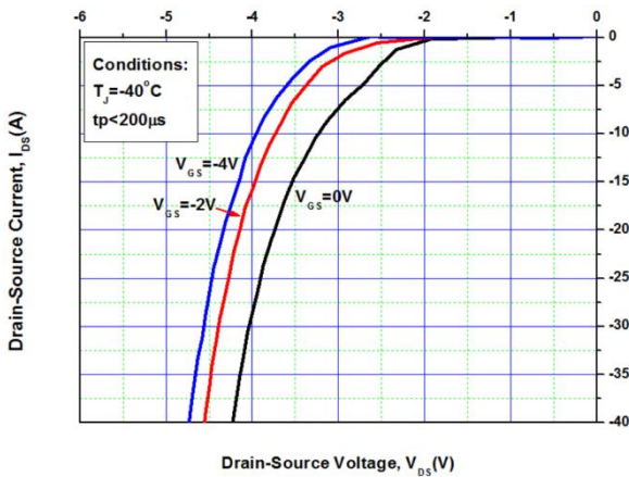
Figure 5. Body Diode Characteristic at -40^\circ\text{C}
