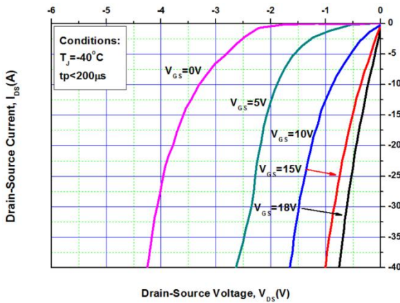
Figure 9. 3rd Quadrant Characteristic at -40°C
