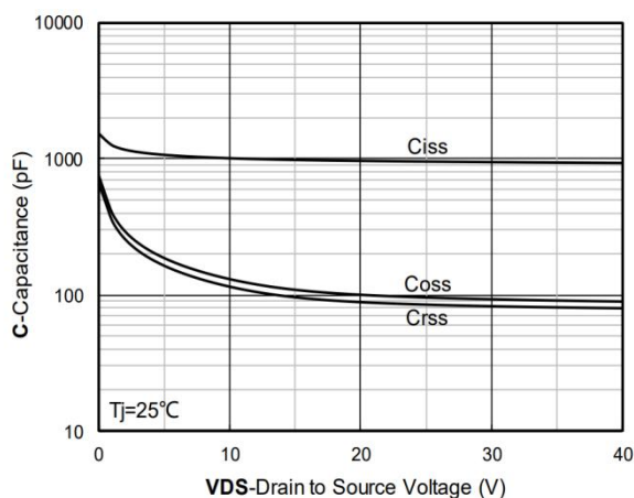
Figure 3. Capacitance Characteristics
