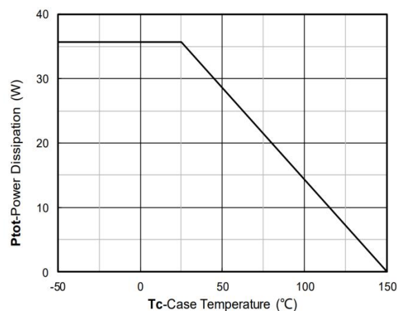
Figure 12. Power dissipation
