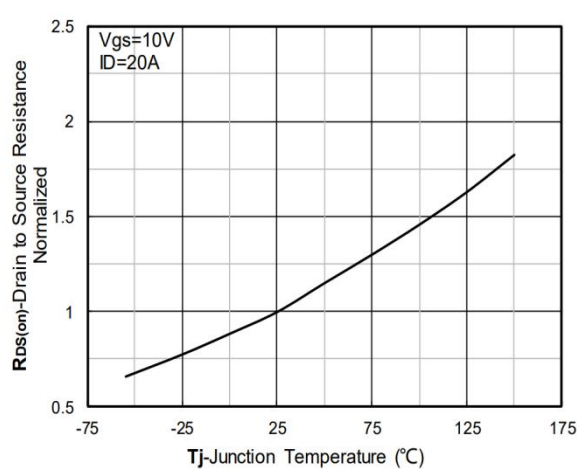
Figure 6. Normalized On-Resistance
