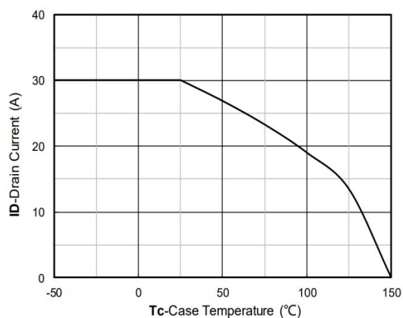
Figure 11. Current dissipation
