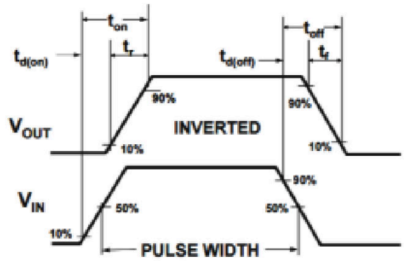
Figure8. Switching wave
