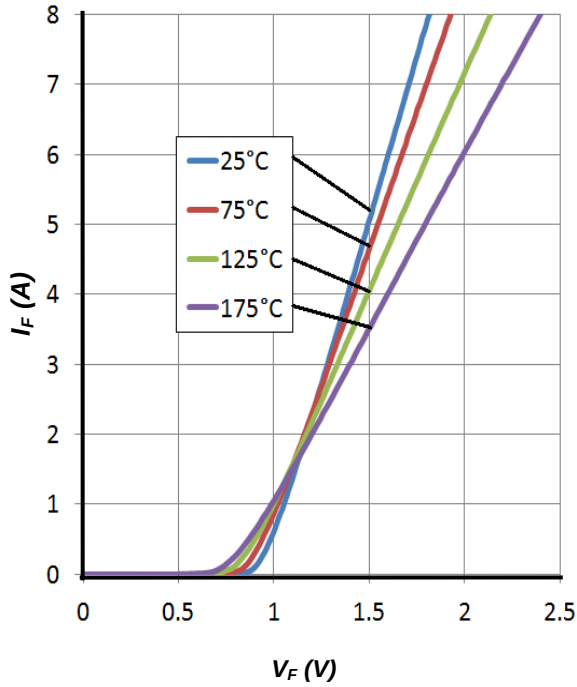
Figure 1. Forward Characteristics
