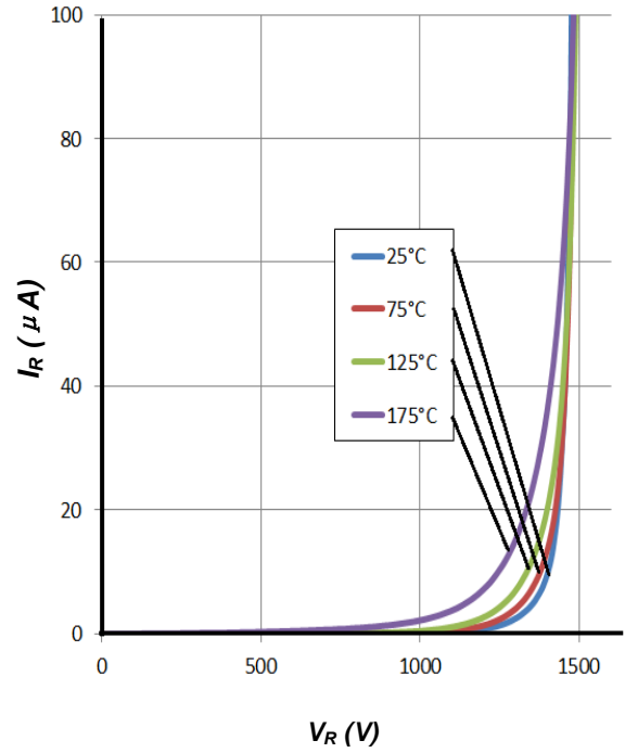
Figure 2. Reverse Characteristics
