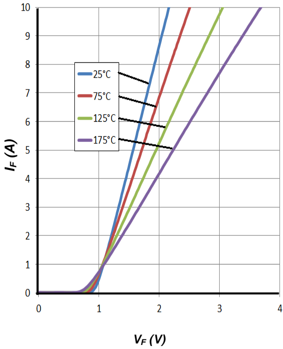
Figure 1. Forward Characteristics
