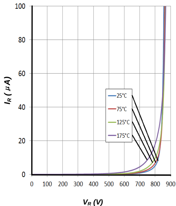
Figure 2. Reverse Characteristics
