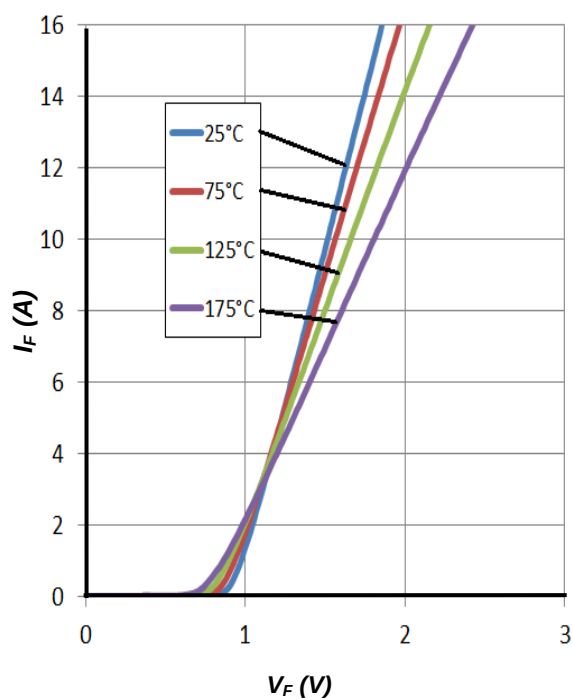
Figure 1. Forward Characteristics
