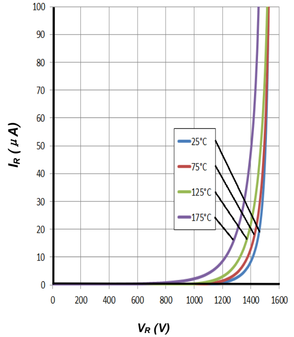
Figure 2. Reverse Characteristics
