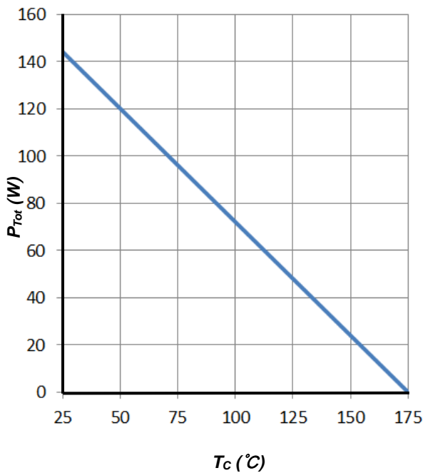
Figure 3. Power Derating
