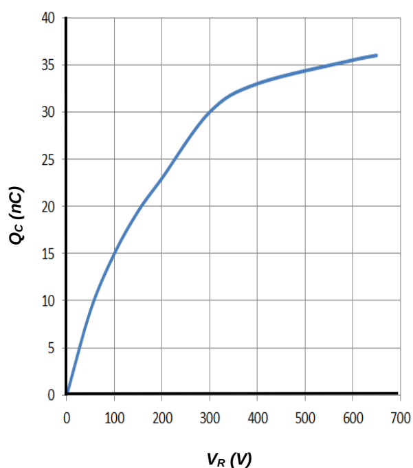
Figure 2. Reverse Characteristics
