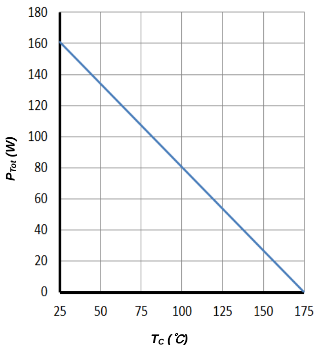
Figure 3. Power Derating
